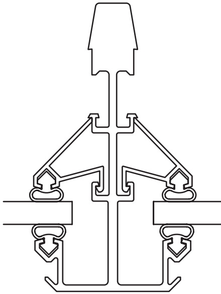
Single Glazing
